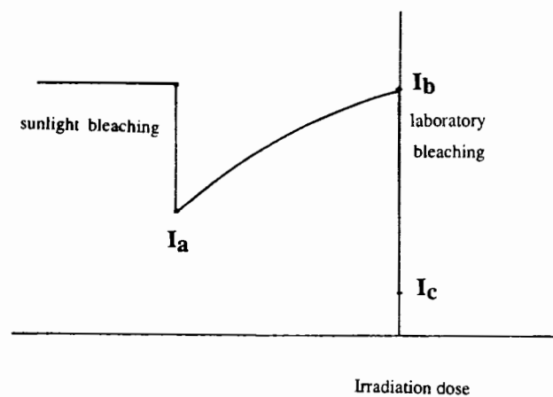
Figure 2. Schematic diagram showing the change in concentration of H-type (the hard to bleach) trapped charges as a result of natural and laboratory bleaching procedures.
