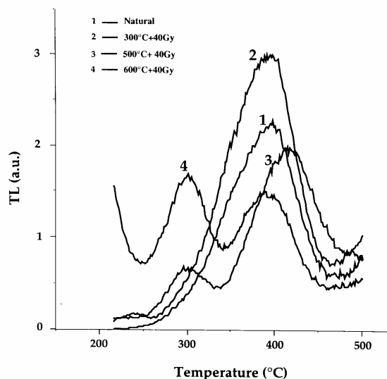
Figure 4. Effect of heating temperature on the TL emission of the raw quartz pebble BPF103
