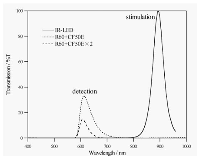
Figure 1. Spectral response of infrared from light emitting diode (LED) for stimulation and filter assemblies for red-IRSL detection.
