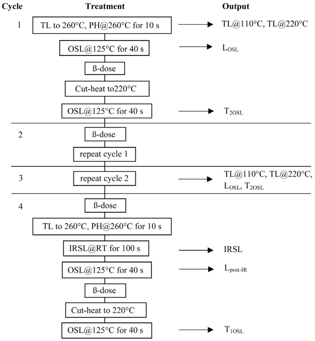
Figure 1: Measurement sequence designed to detect feldspar contaminants. For TL@110°C, TL@220°C, L OSL and T 2OSL the output of cycle 3 was used, and for IRSL, L post-IR and T 1OSL the output of cycle 4 was used. Equal laboratory regenerative doses of ~10 Gy were administered in each cycle.
