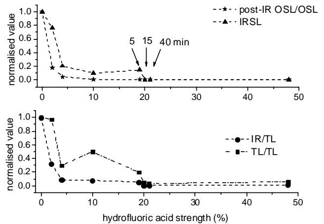
Figure 5: Comparison of the feldspar contamination tests for sample LV 01. The plots display the normalised values (calculated as described in the Fig. 4 caption) versus HF strength. The time difference of treatment with 20% HF (5, 15 and 40 min) is depicted by three data points centred on 20% HF strength. IRSL and TL/TL show a relatively high sensitivity to feldspar contamination whereas IR/TL and [post-IR] OSL/OSL seem to be less sensitive.
